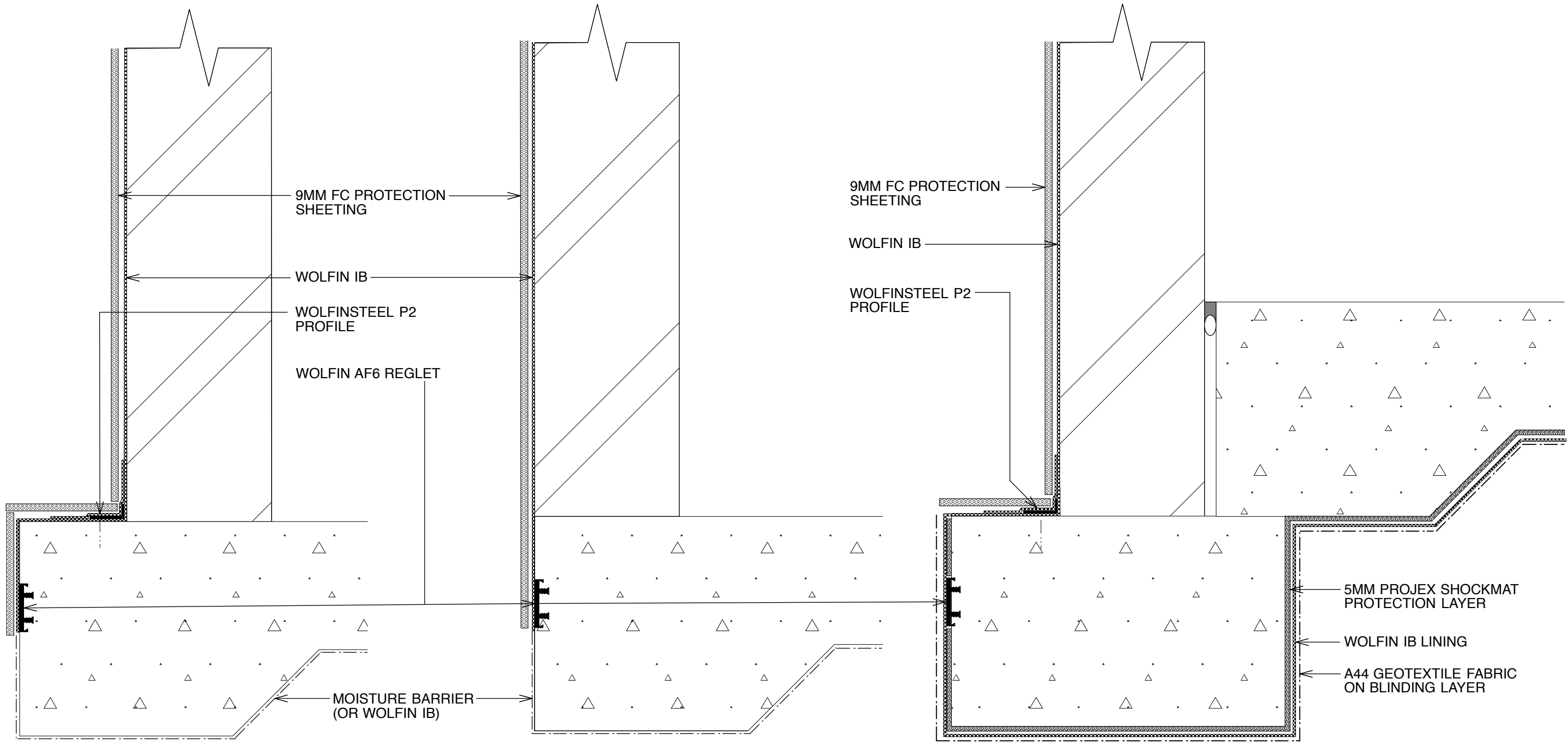
SECTION: BASEMENT WALL ON SLAB JUNCTION DETAIL - OFFSET
