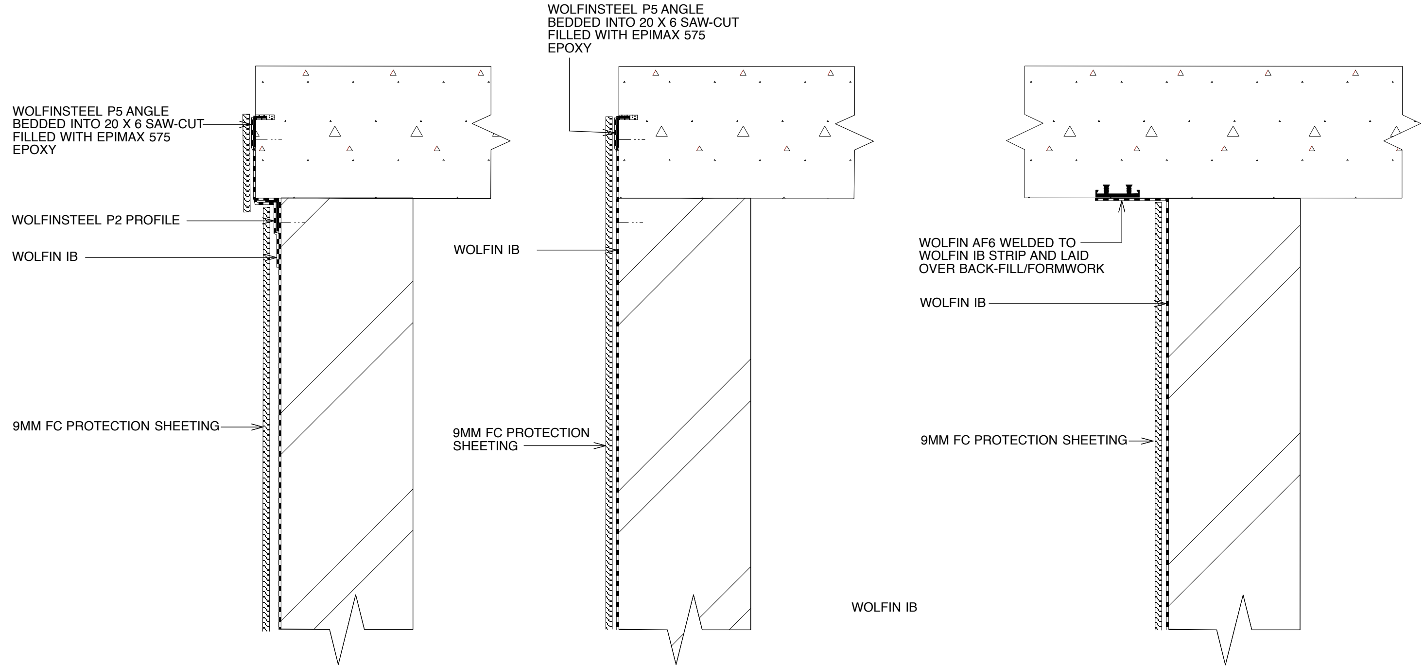
SECTION: BASEMENT WALL/GROUND FLOOR JUNCTION DETAIL - OFFSET
