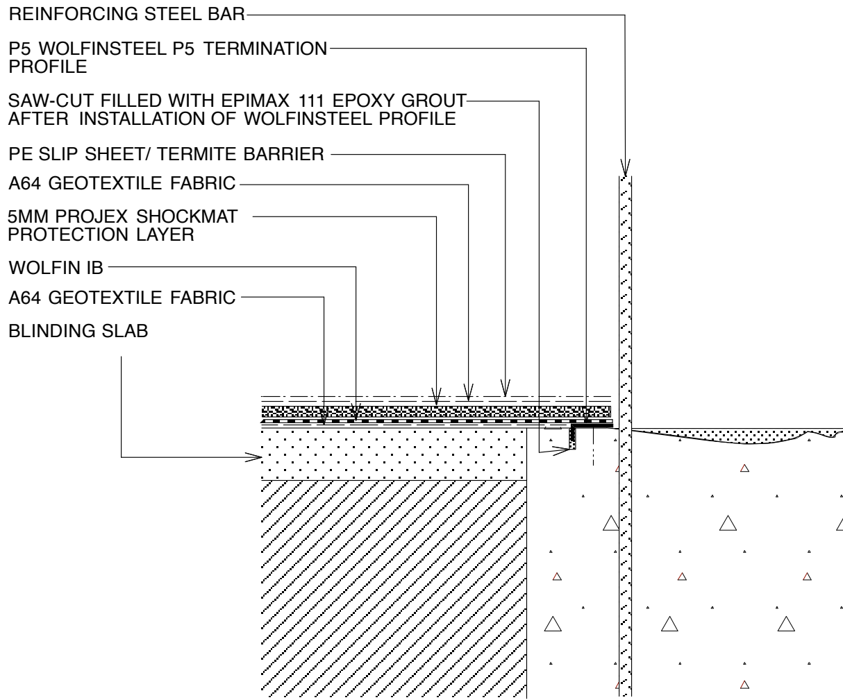
DETAIL: PILE CAP - HALF SECTION
